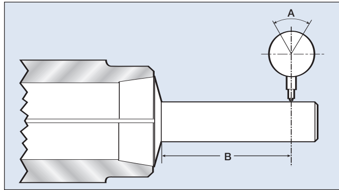
Accuracy chart for Crawford Drawback Collets
